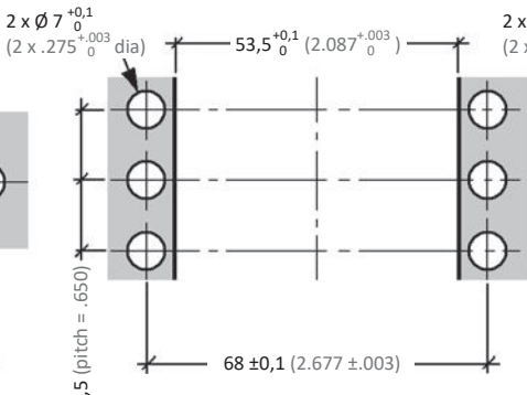
Perçage multiple Multiple cutout
