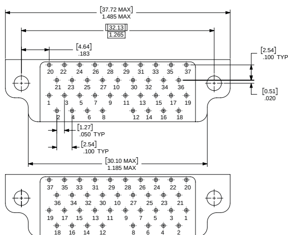
37 CONTACTS
