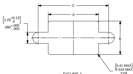
FIGURE 1 SIZE 9-69 FRONT MOUNTING
