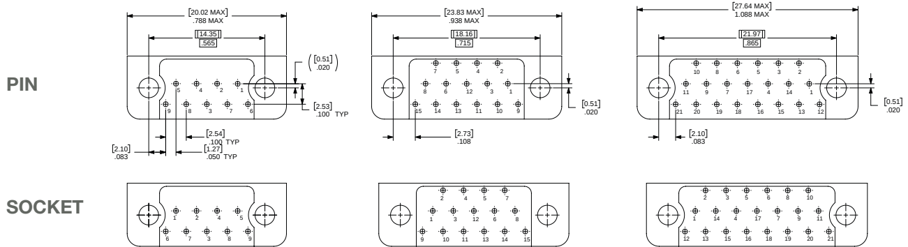
9 CONTACTS
