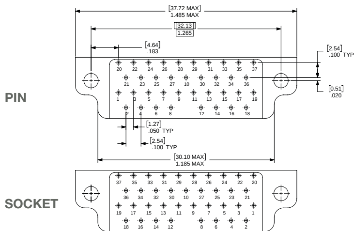
37 CONTACTS
