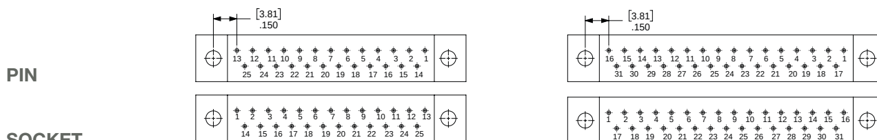
25 CONTACTS
