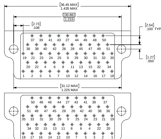
51 CONTACTS
