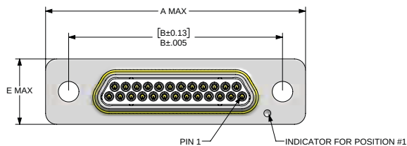
PLUG
