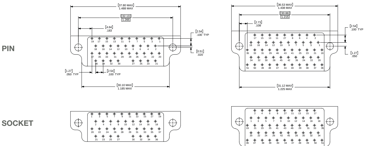
37 CONTACTS
