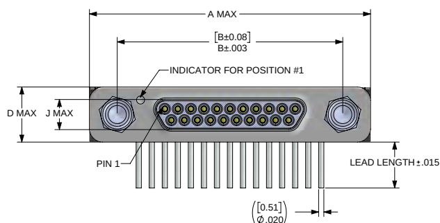
PLUG
