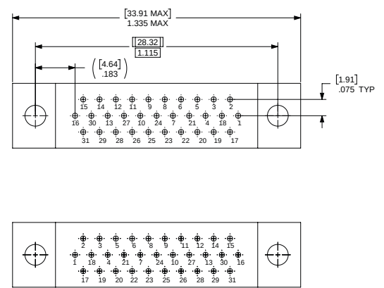
31 CONTACTS
