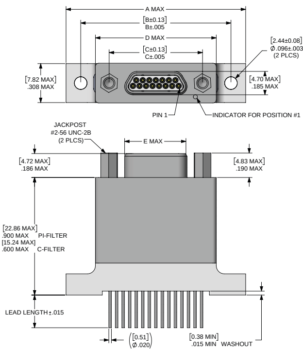
PLUG
