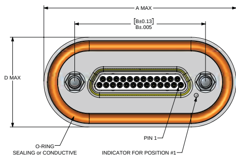
PLUG
