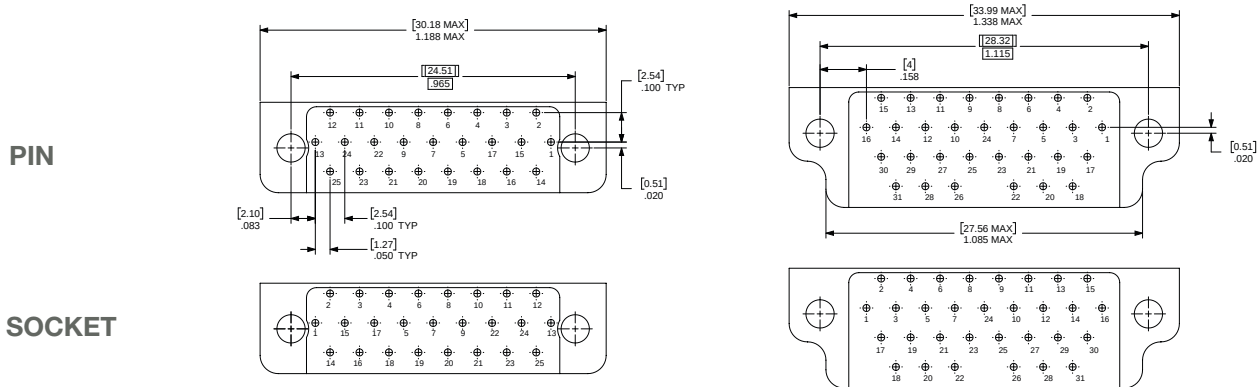
25 CONTACTS
