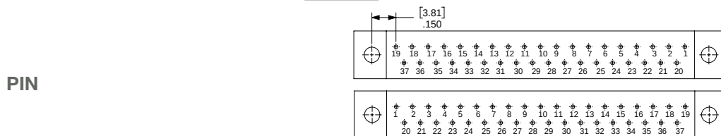
37 CONTACTS
