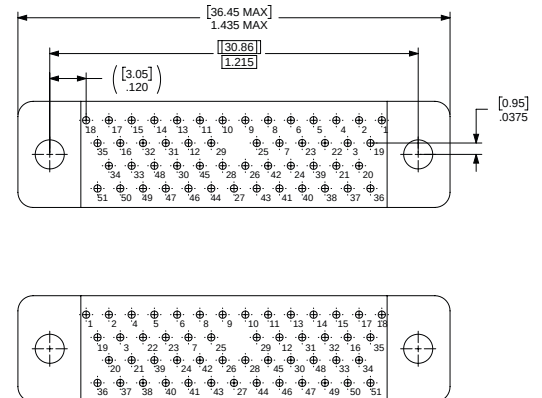
51 CONTACTS
