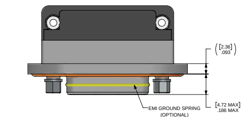
PLUG
