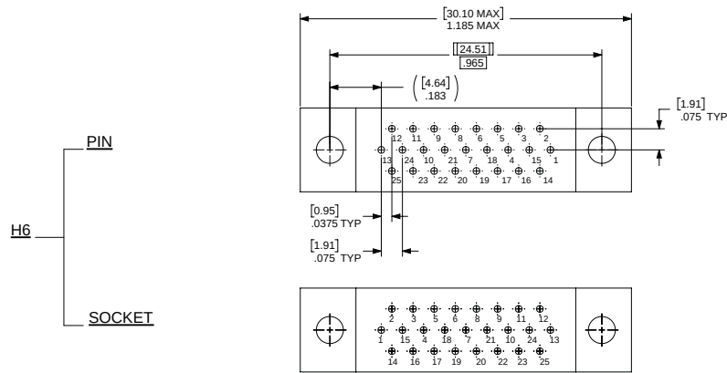
25 CONTACTS
