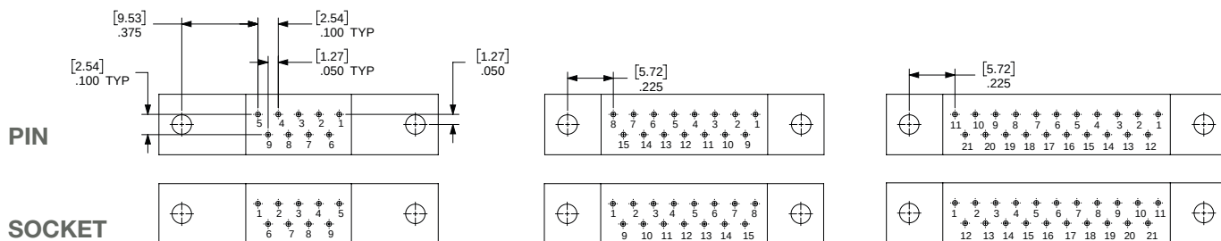
9 CONTACTS
