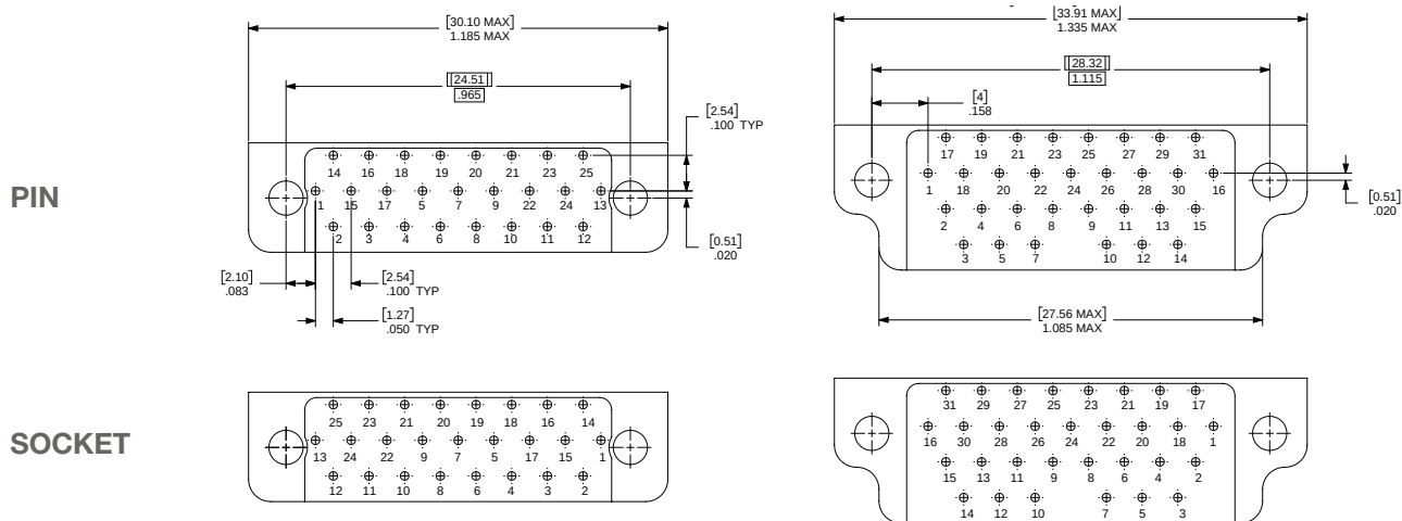
25 CONTACTS
