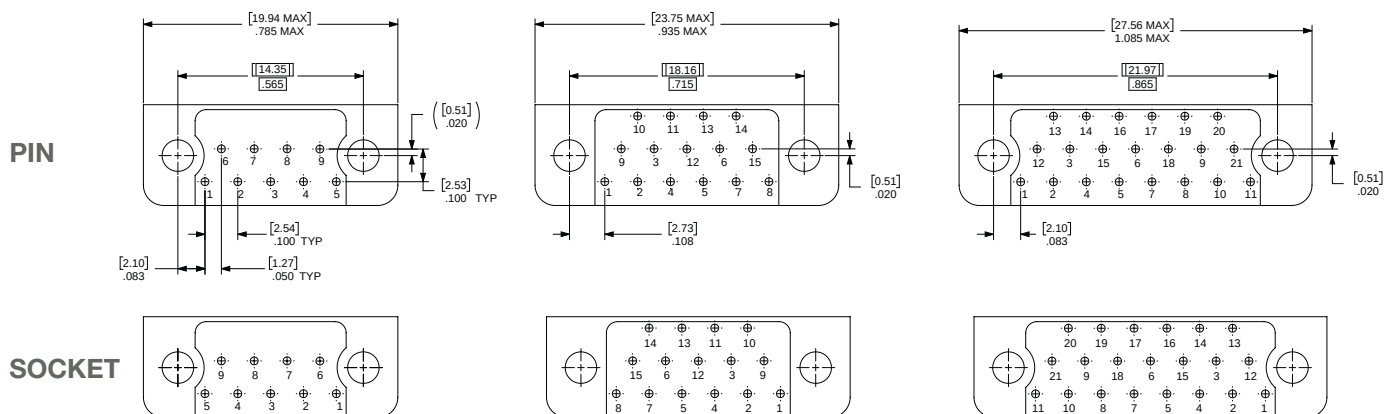
9 CONTACTS
