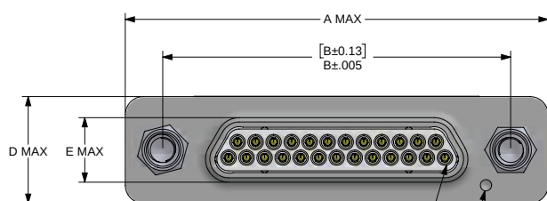
PLUG
