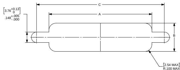
FIGURE 4 SIZE 100 REAR MOUNTING
