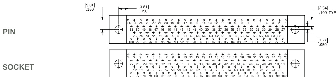
100 CONTACTS
