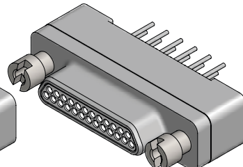
Slot Head-Short
