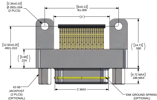
PLUG
