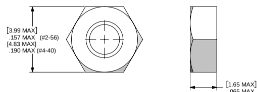
Nut Detail
