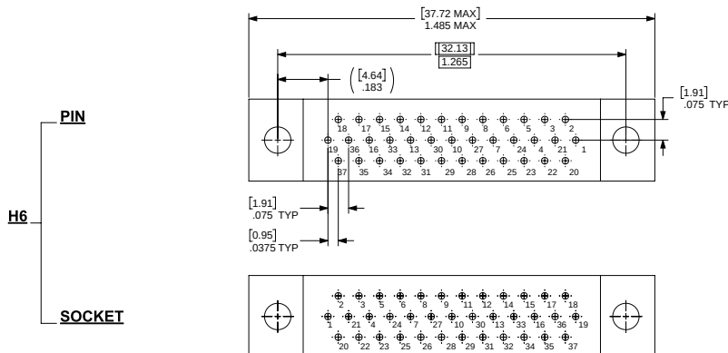
37 CONTACTS
